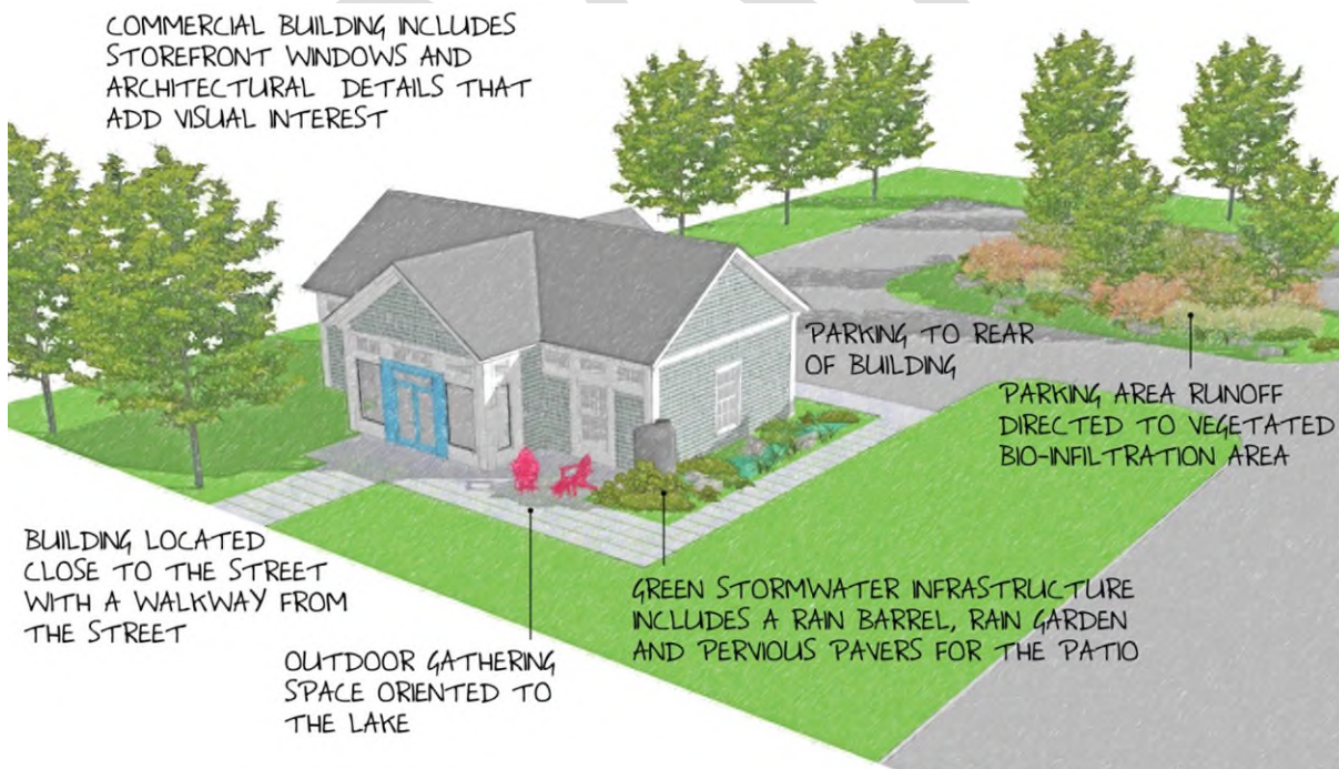
Figure 4-2. Building Placement and Design Standards Illustrated
