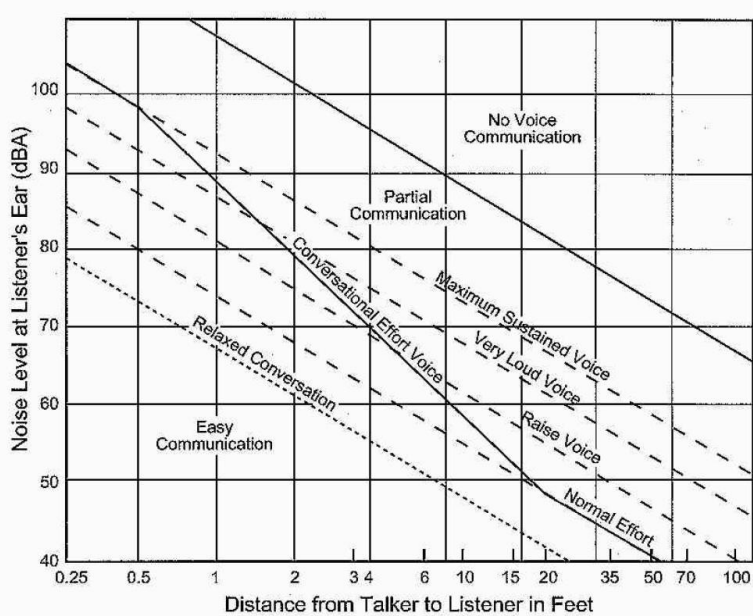
Figure 3-1. Speech interference.
