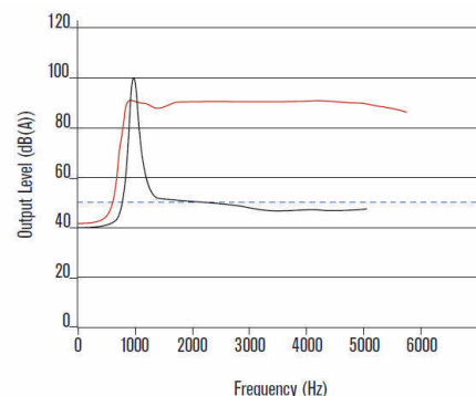
Figure 6-1. Frequency spectrum of backup alarms
