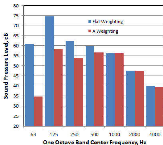
Figure C-6. Flat and A-weighted frequencies
